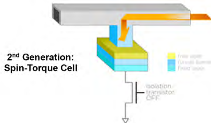
Figure 3.2-6. ST-MRAM 1T/1MTJ memory cell [17].
