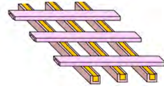
Figure 4.4-1. Cladding (pink) surrounding magnetic traces is sensitive to stray magnetic fields [18].
